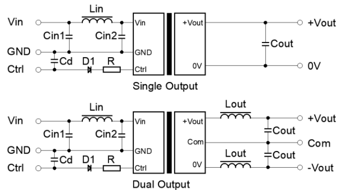
Figure 1: Typical External Circuit
